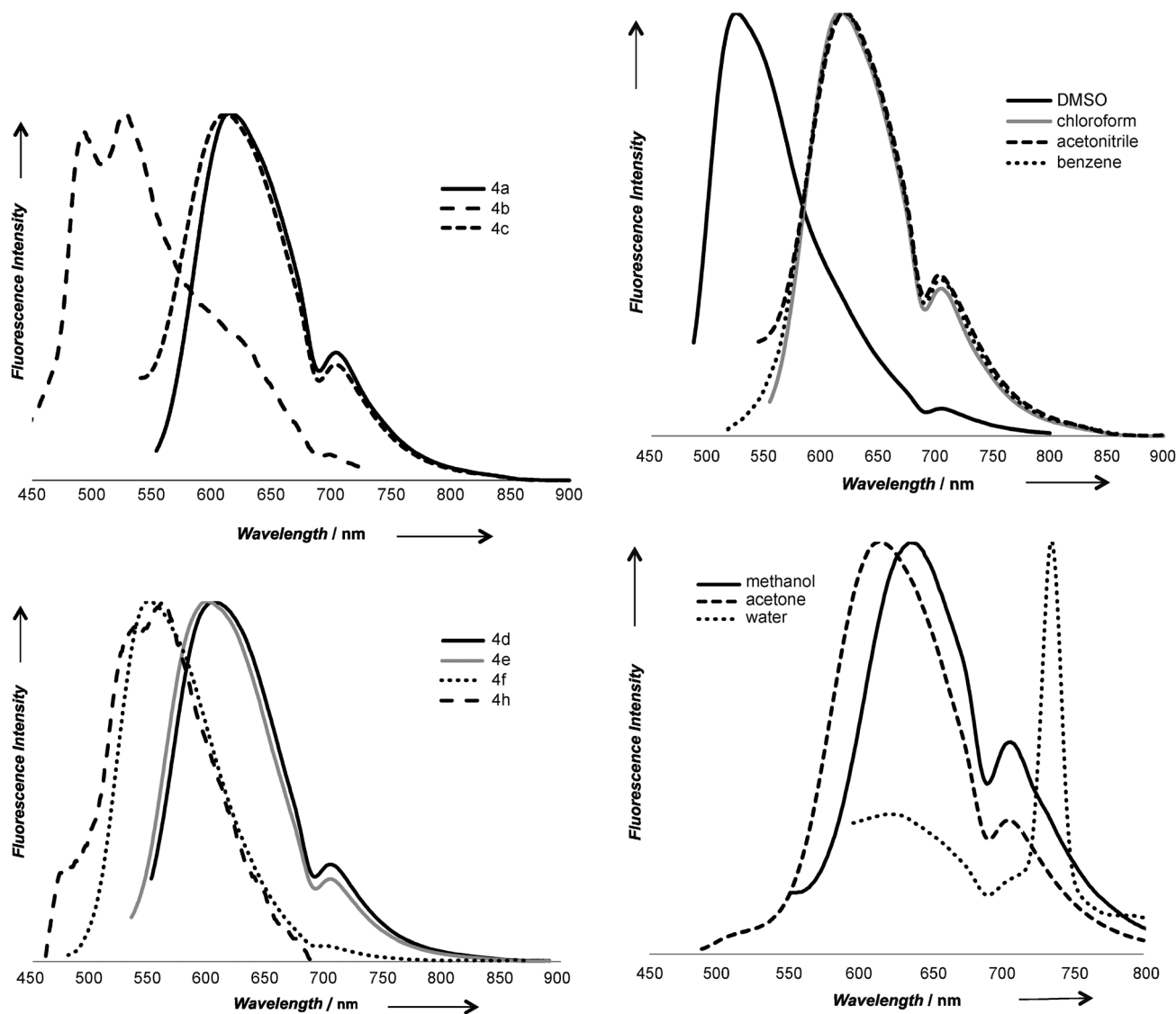
Figure 3. Fluorescence spectra of compounds 4 in chloroform.
