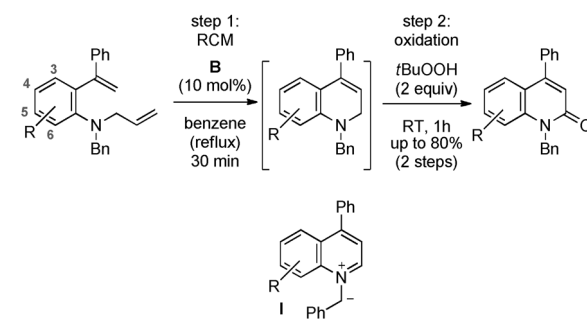
Scheme 1. One-pot RCM/oxidation reaction. Bn = benzyl.
